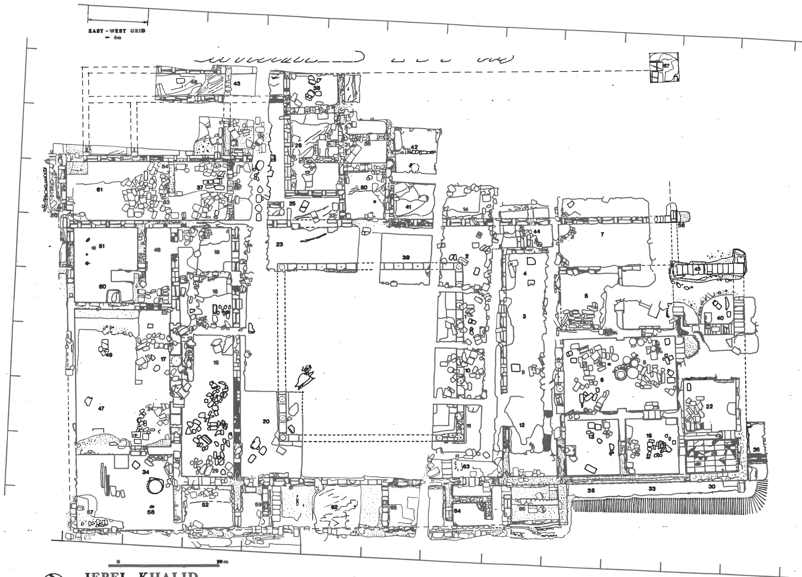
JEBEL KHALID ACROPOLIS PALACE · GROUND PLAN 1996
